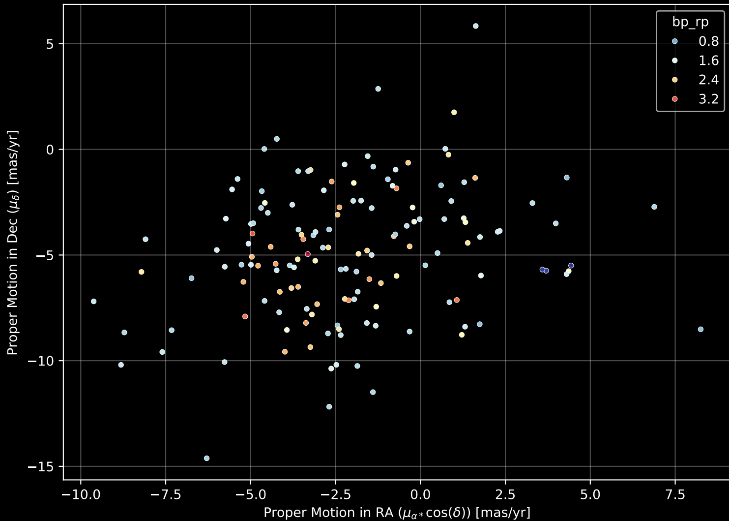
APOGEE DR17 Field: [356-04-O] Proper Motion Diagram (n= 146)
