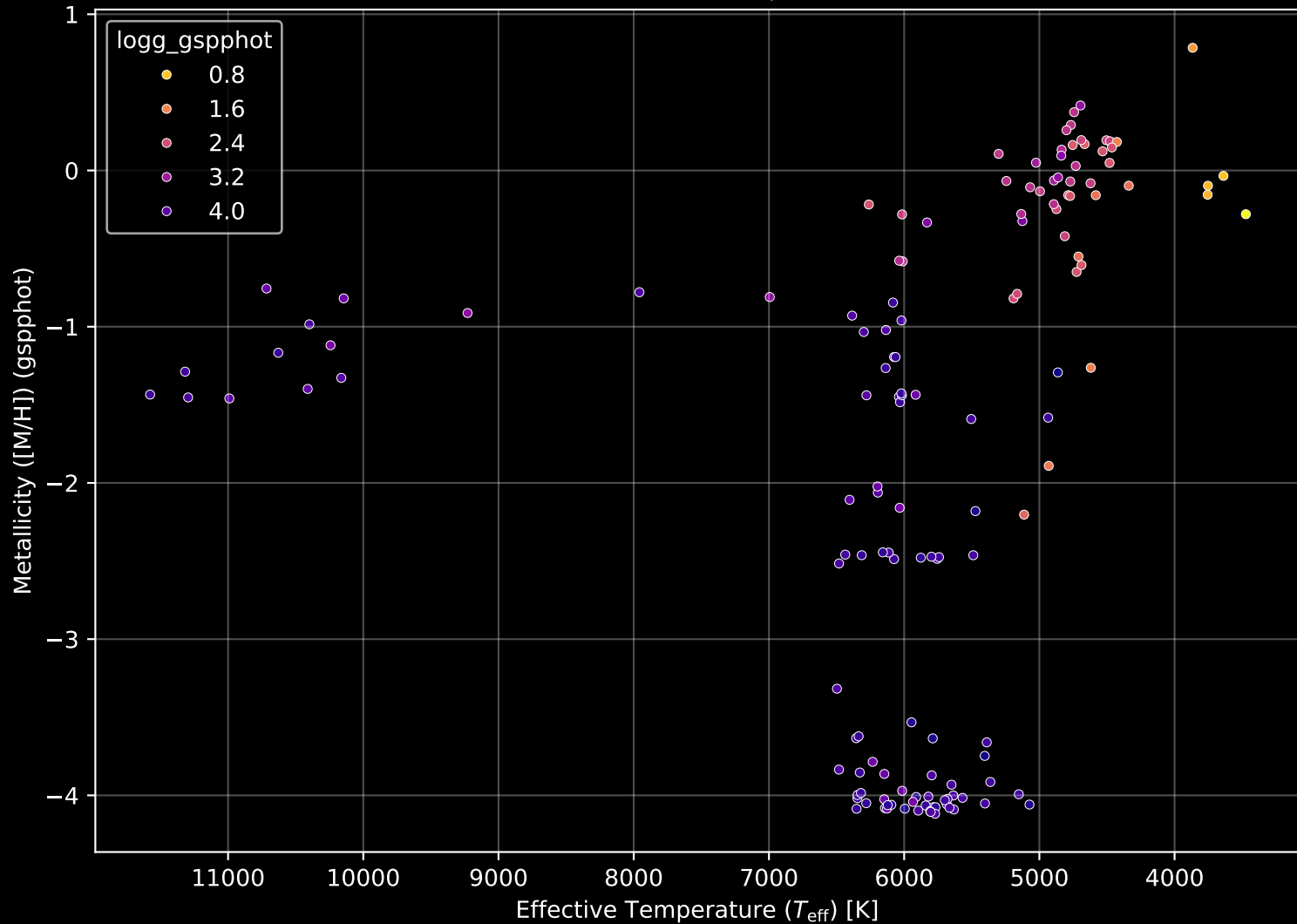
APOGEE DR17 Field: [356-04-O] Stellar Population Parameters (n= 146)
