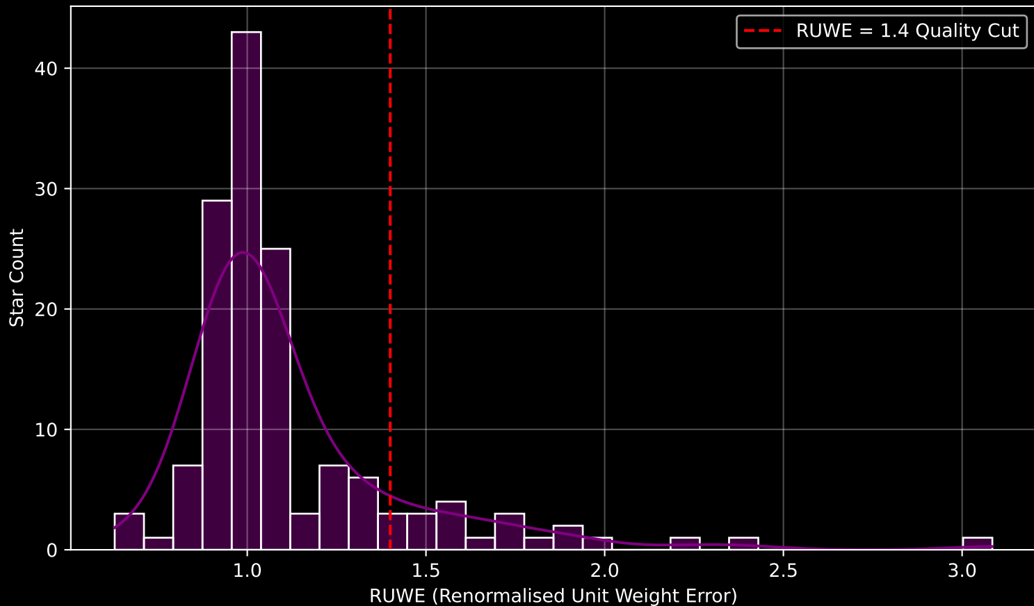
GAPOGEE DR17 Field [356-04-O] RUWE Distribution (n= 145)
