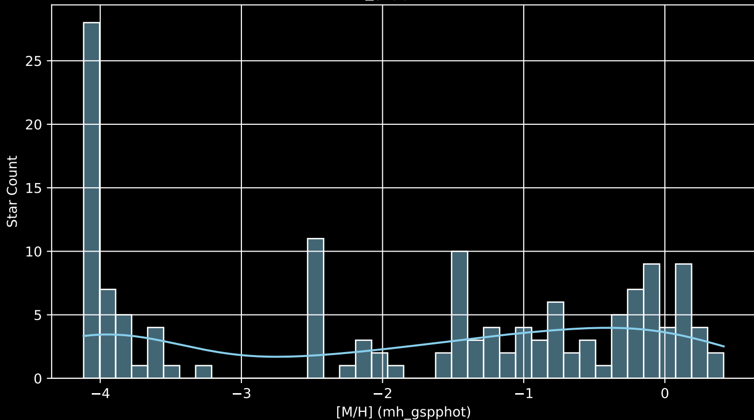
APOGEE DR17 Field: [356-04-O [M/H] (mh_gspphot) (n= 145)
