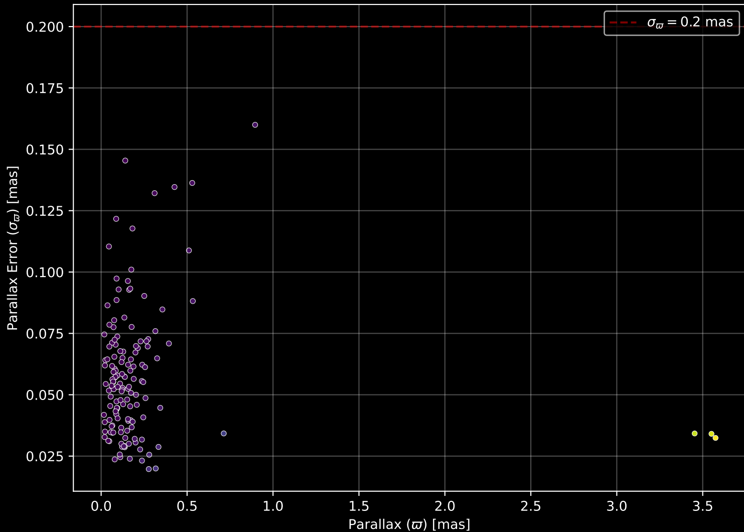
APOGEE DR17 Field: [356-04-O] Parallax Quality (n= 146)
