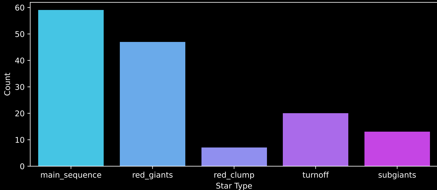
APOGEE DR17 Field: [356-04-O] Count plot of Star Type
