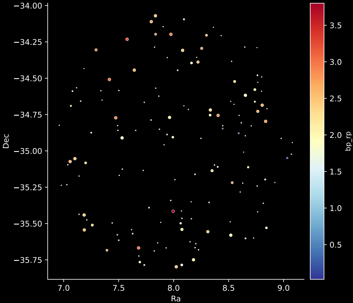
APOGEE DR17 Field: [356-04-O] Stars: 146
